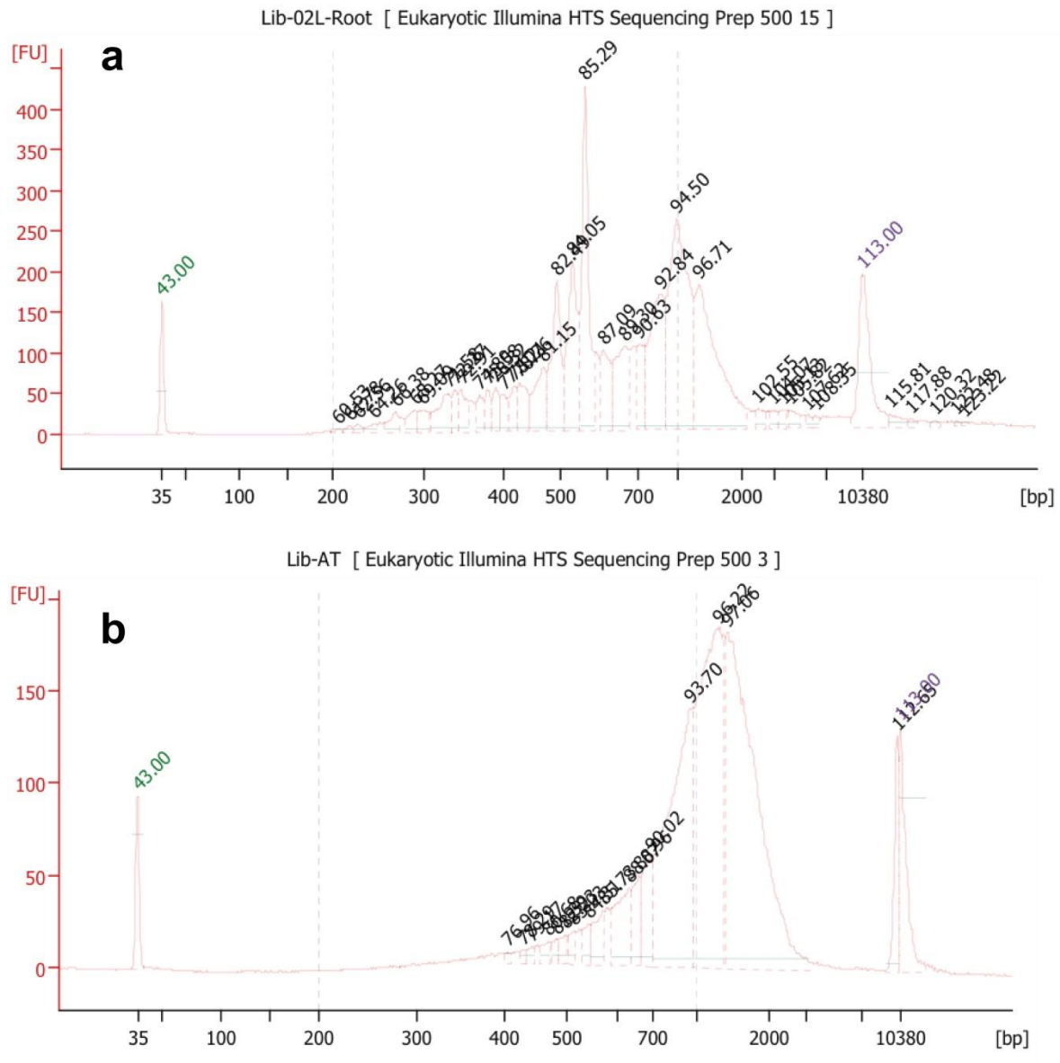
Figure S1. Effect of rRNA depletion on nanoCAGE-XL library profile
